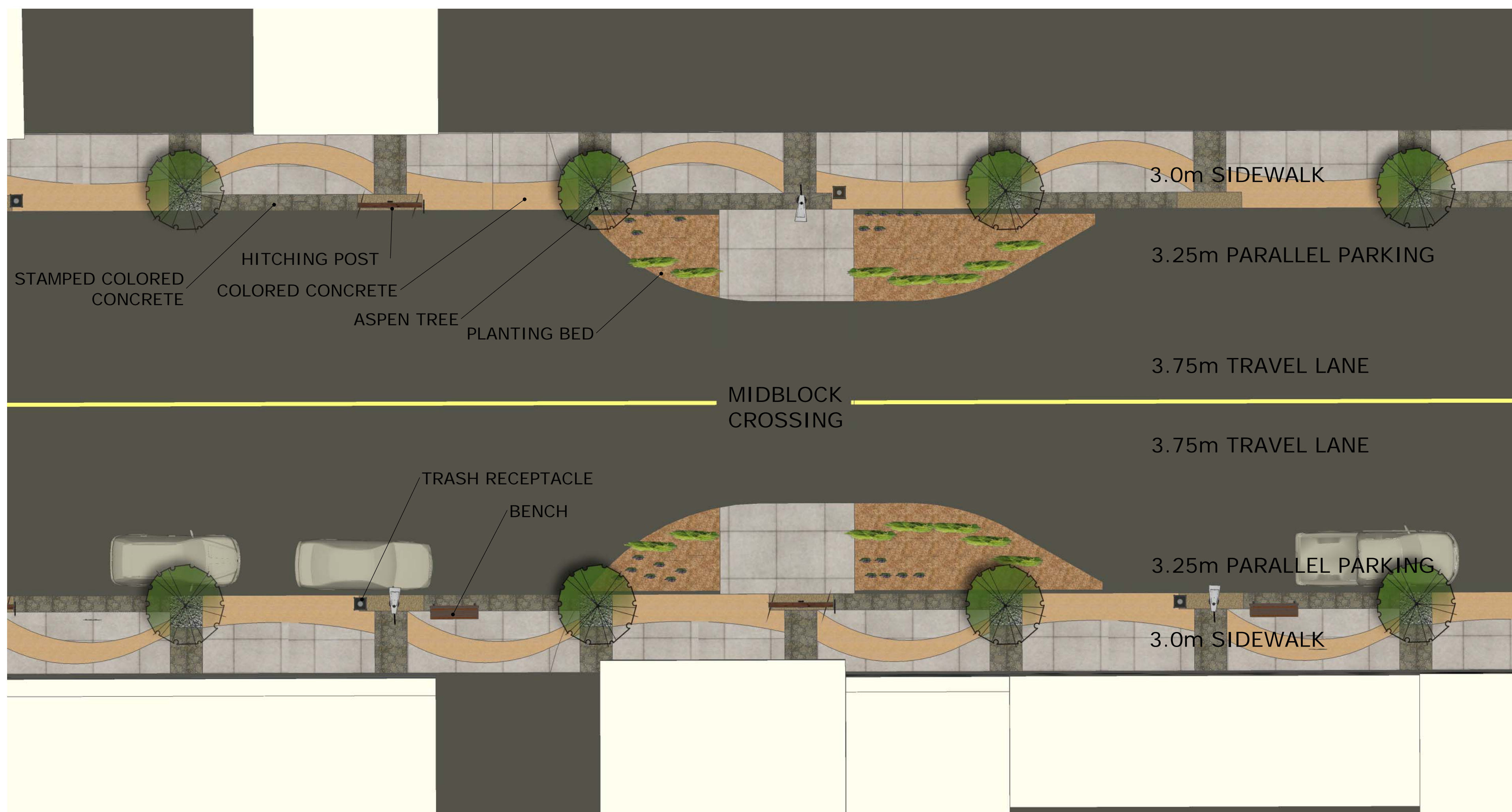
PLAN VIEW
